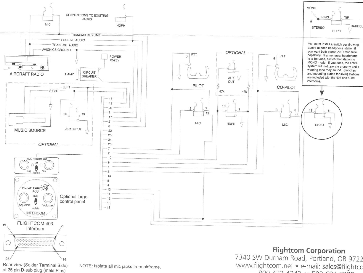
Figure 6 - Connection Schematic - Mono Mode
