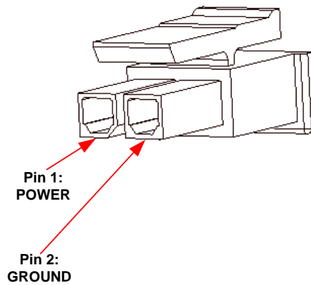
Figure 3: Harness
