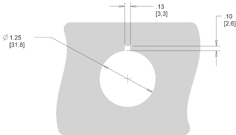
Figure 1: Mounting location
