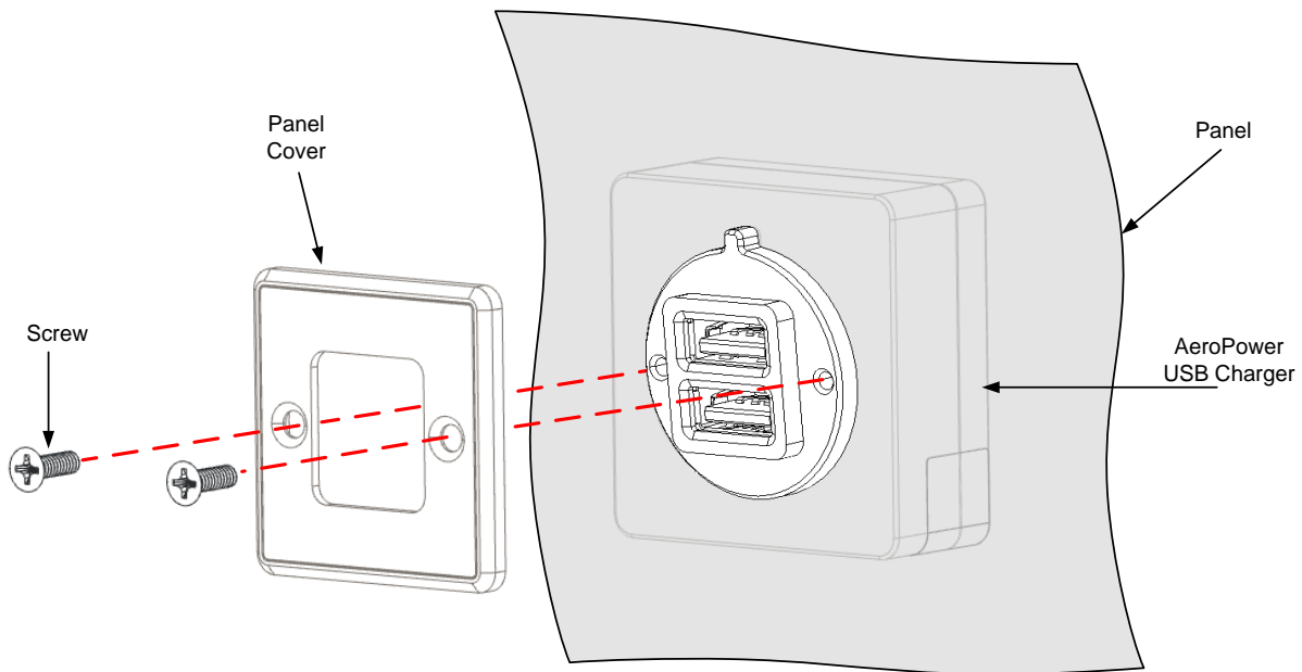
Figure 2: Installing AeroPower USB Charging Port
