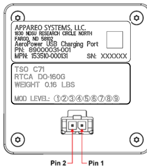
Figure 4: Back of AeroPower
