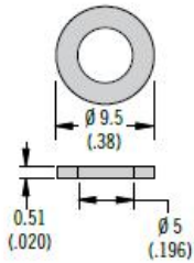
Sealing Washer
