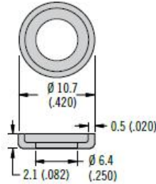
Cupped Washer
