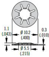
Retainer Push-On
