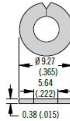
Retainer Split
